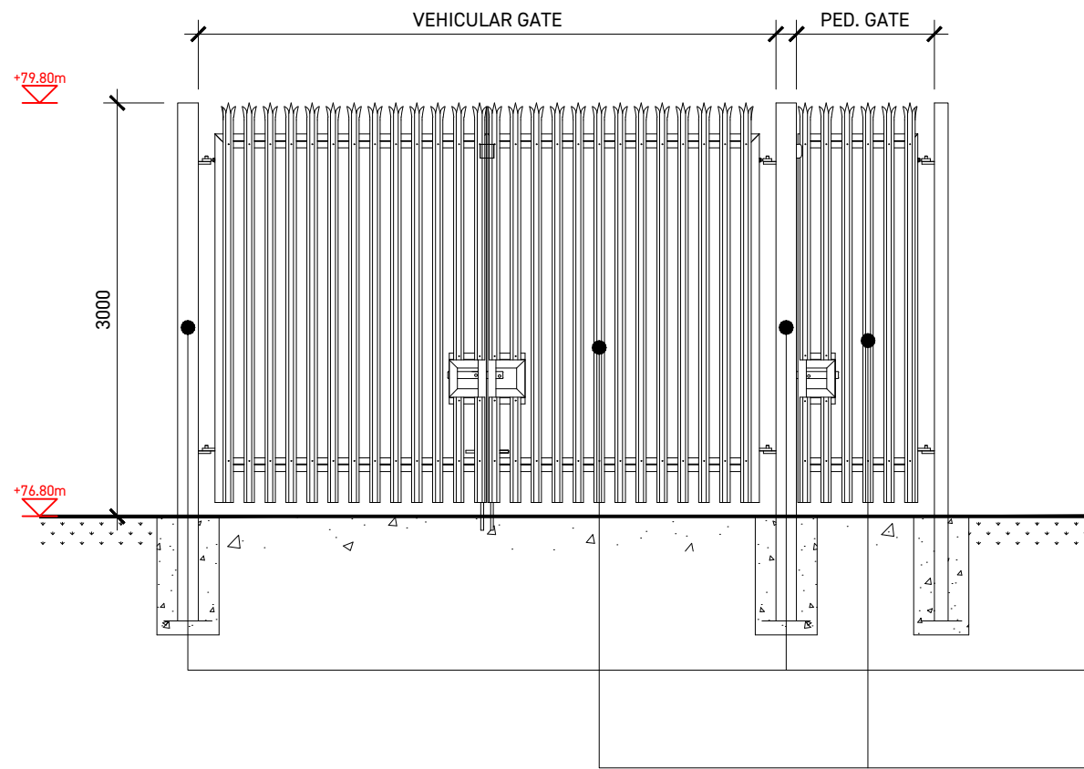
PALISADE GATE ELEVATION
