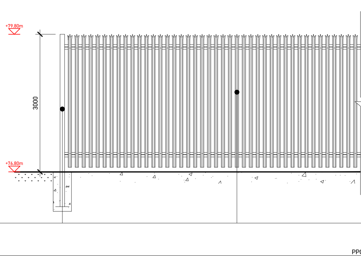
PALISADE FENCE ELEVATION
